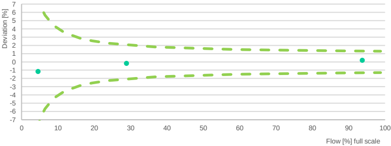
Example: typical measuring points of a 3-point calibrated Flowmax in error graph according definitions
