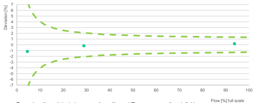
Example: allowed deviation area of a calibrated Flowmax according to definitions
